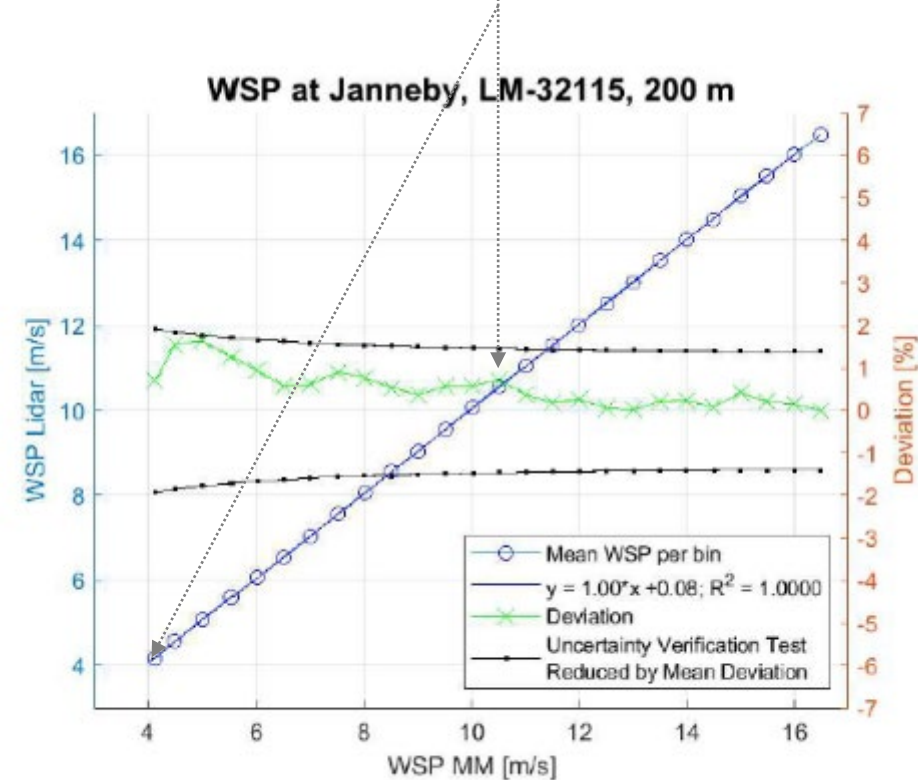
Figure 14: Scatterplot bin-wise wind speed and deviation at 200 m
